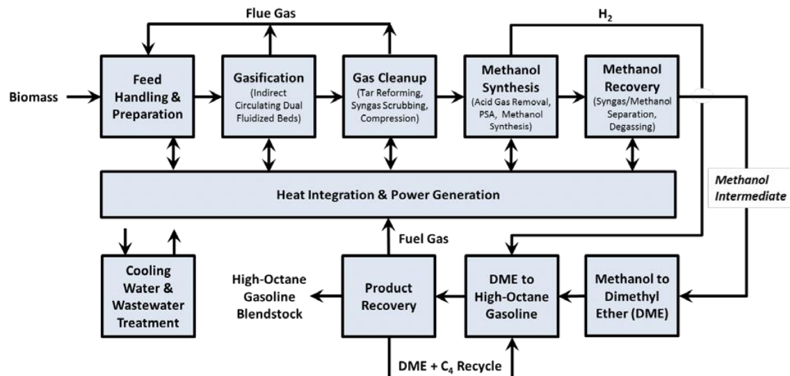
Figure 1: Production of High-Octane Gasoline Blendstock via Syngas Conversion Pathway and Methanol/Dimethyl Ether Intermediates
